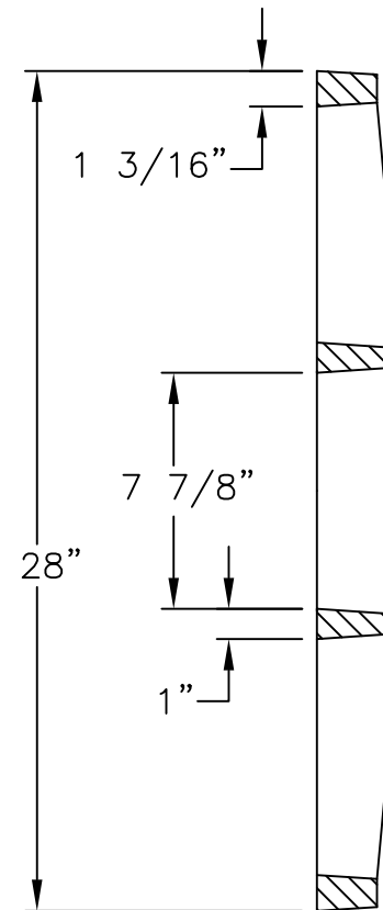
GRATE SECTION
