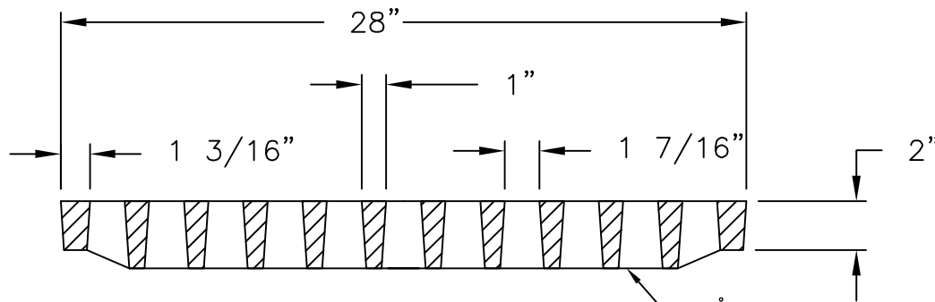
GRATE SECTION
